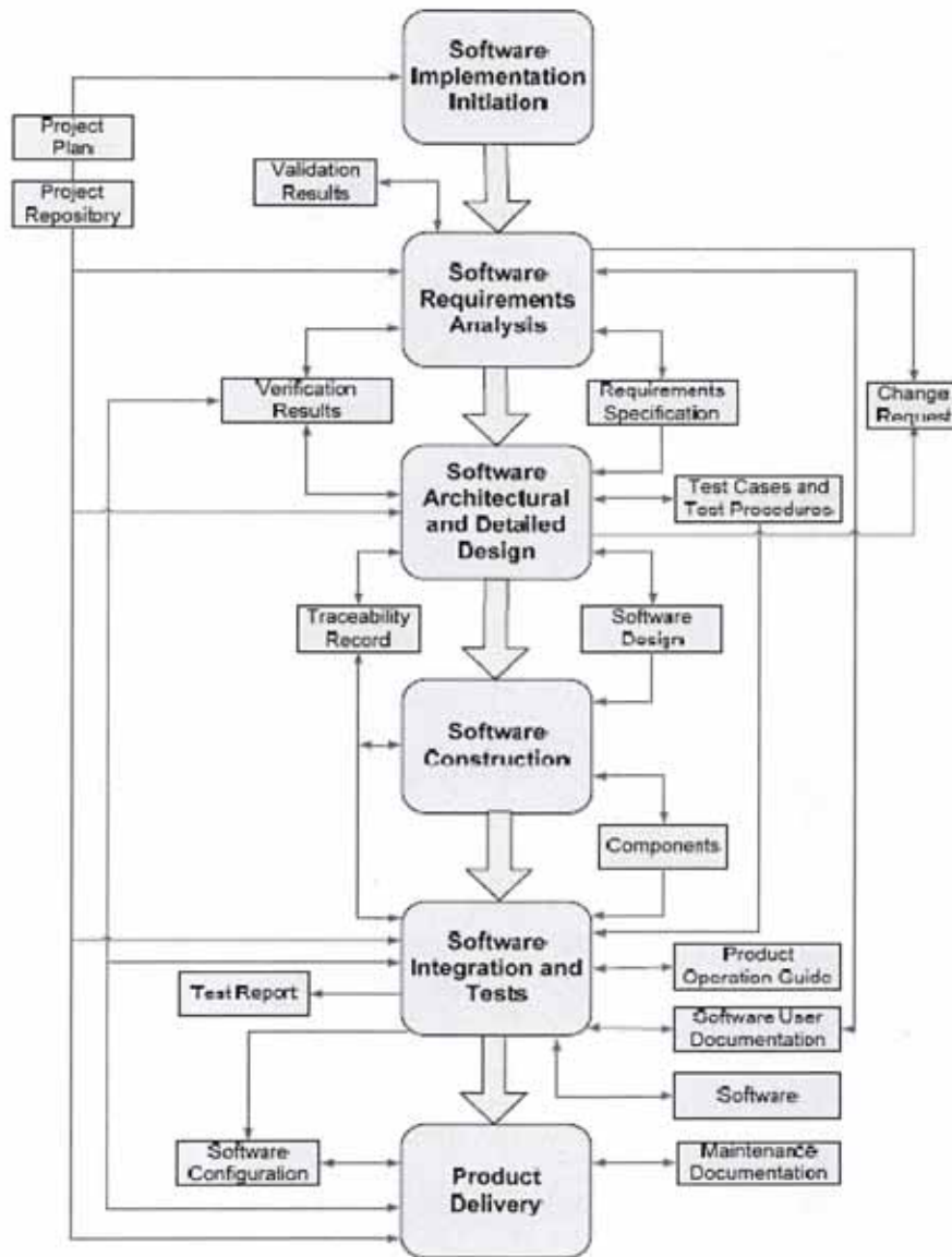
Software Implementation Process Diagram
